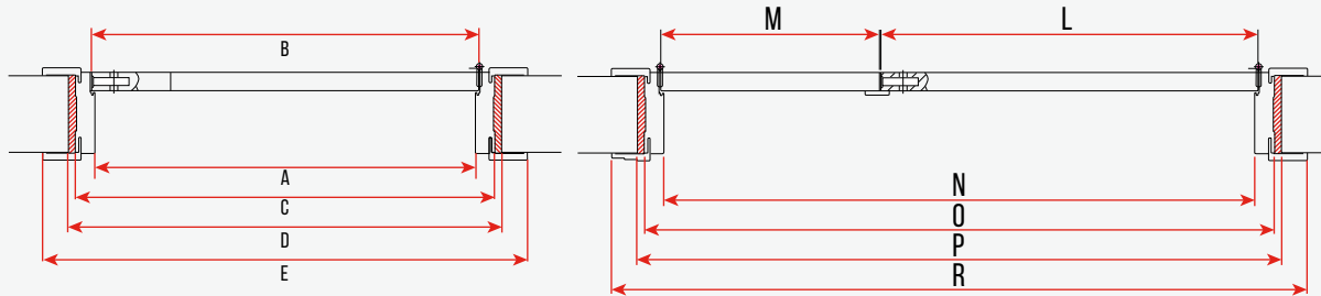
RESİM/PICTURE 1: KAPI GENEL KESİT DOOR'S GENERAL CROSS SECTION
